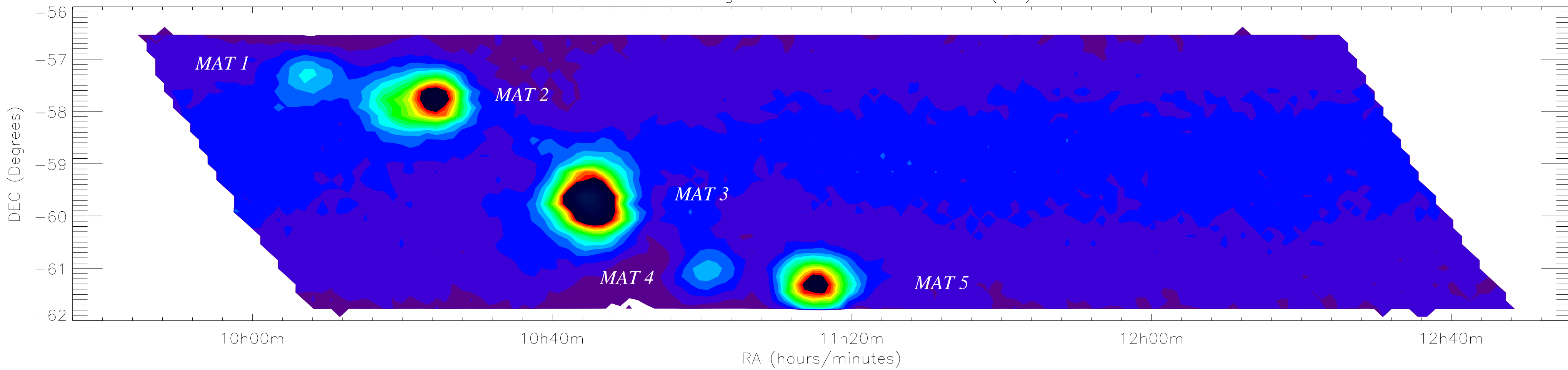
Galactic Region Observed at 40 GHz (Q1)
